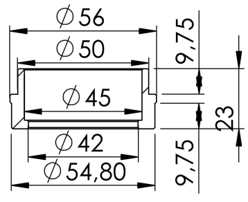
"Bushing" Cod.206424
