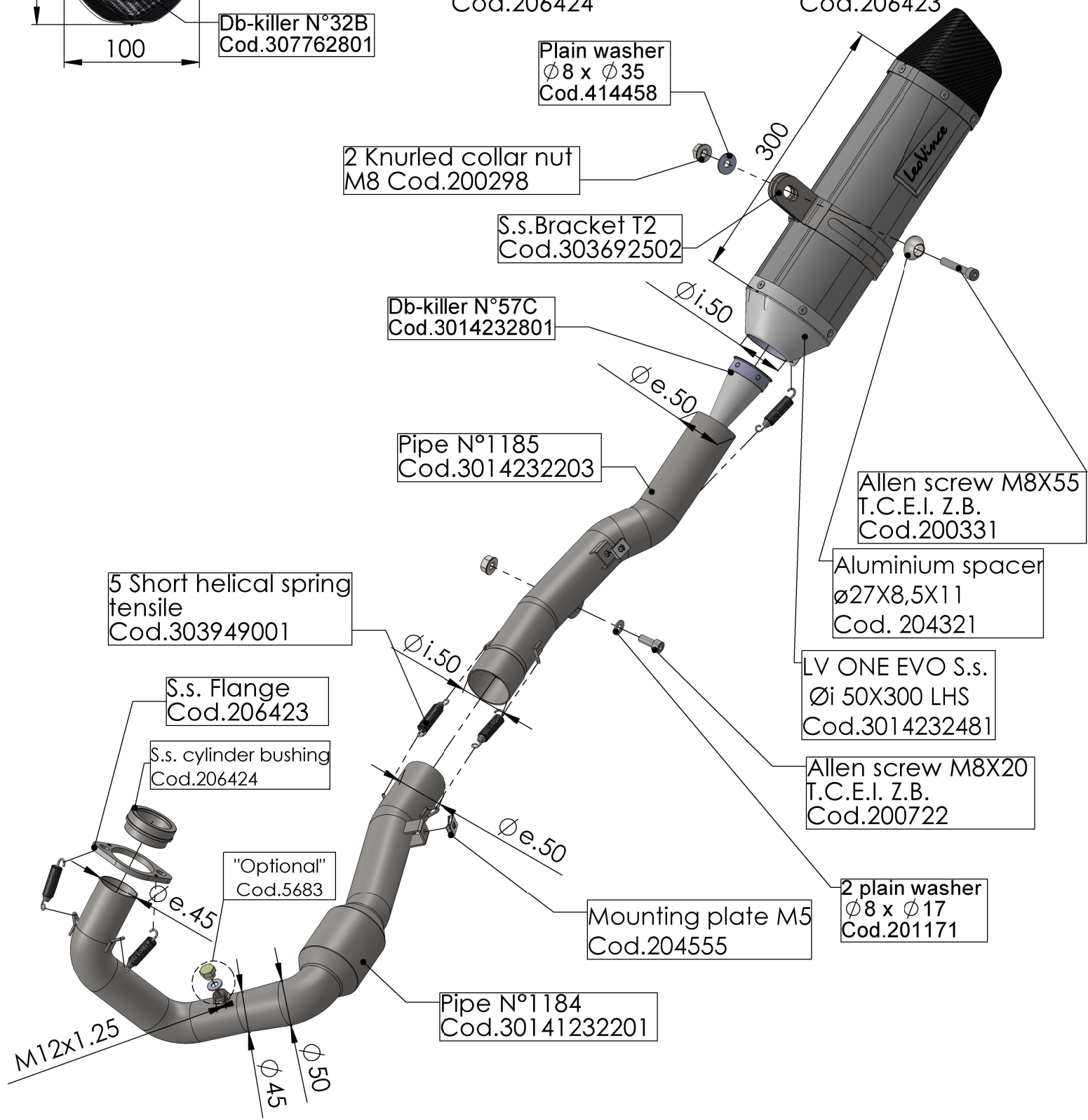
"Bushing" Cod.206424
